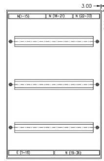
FRONT VIEW FRONT COVER NOT SHOWN
