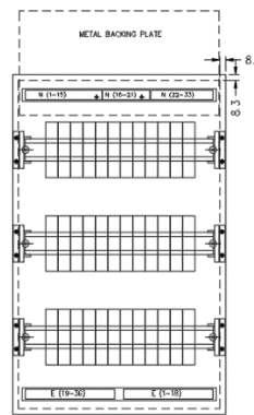
FRONT VIEW FRONT COVER NOT SHOWN
