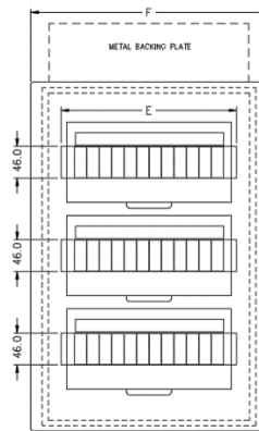
FRONT VIEW FRONT DOORS NOT SHOWN
